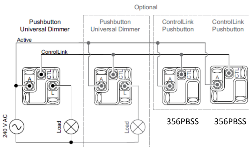
Wiring Diagram – for Multiway dimming
