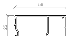
ASL 896 132mm GLAZING BEAD
