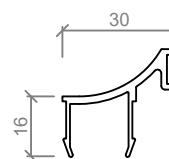
ASL 901 POCKET DOOR STOP UP TO 45mm DOOR
