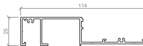
ASL 895 132mm GLAZING BAR
