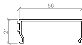
ASL 894 TRANSOM BEAD
