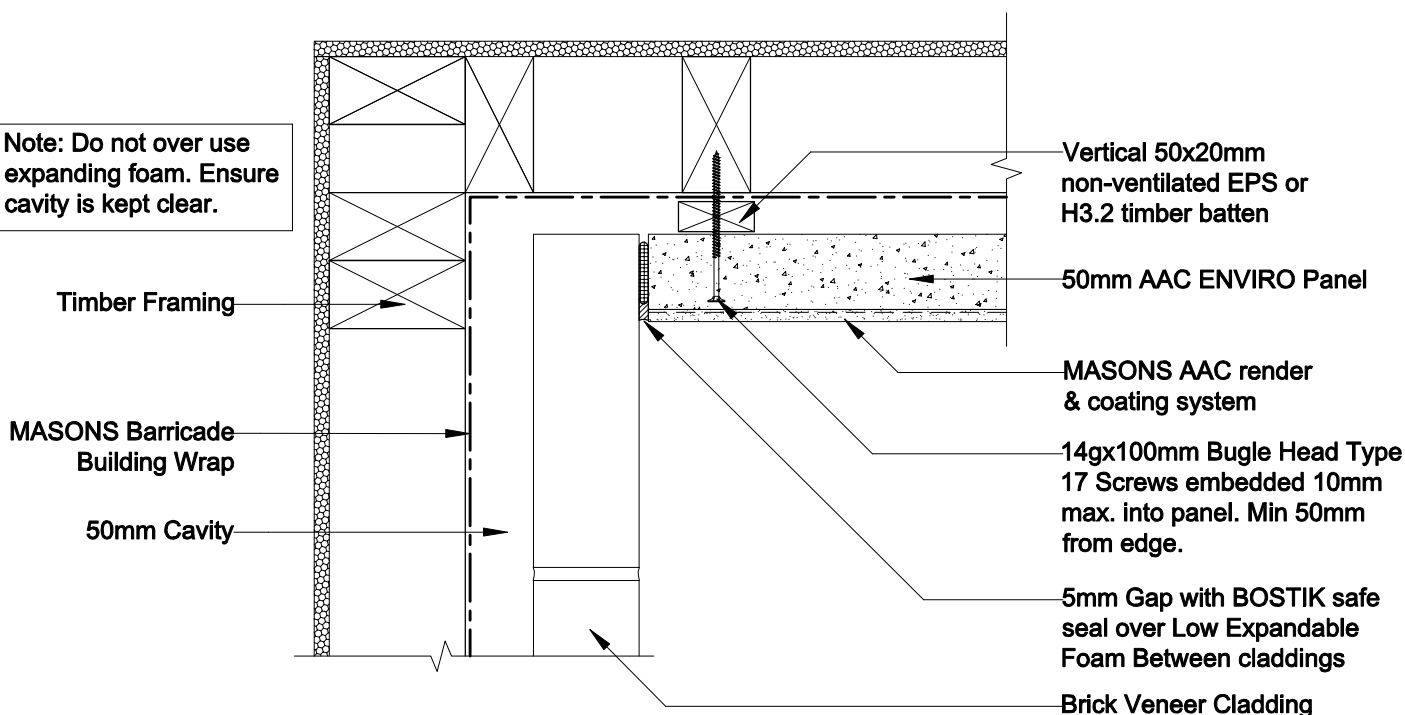
Detail 43 Scale 1:5
