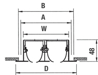
Dimensions - Diffuser Only
