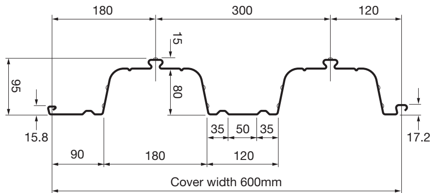
ComFlor 80 Composite Slab - Volume & Weight
