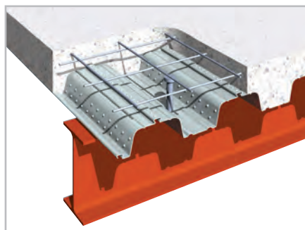
ComFlor 80
