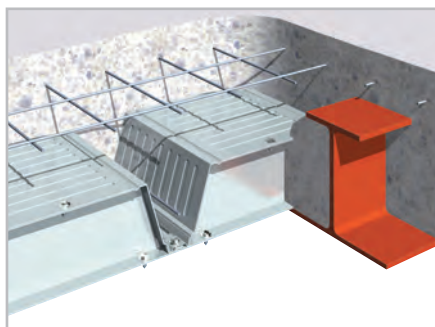
ComFlor 210
