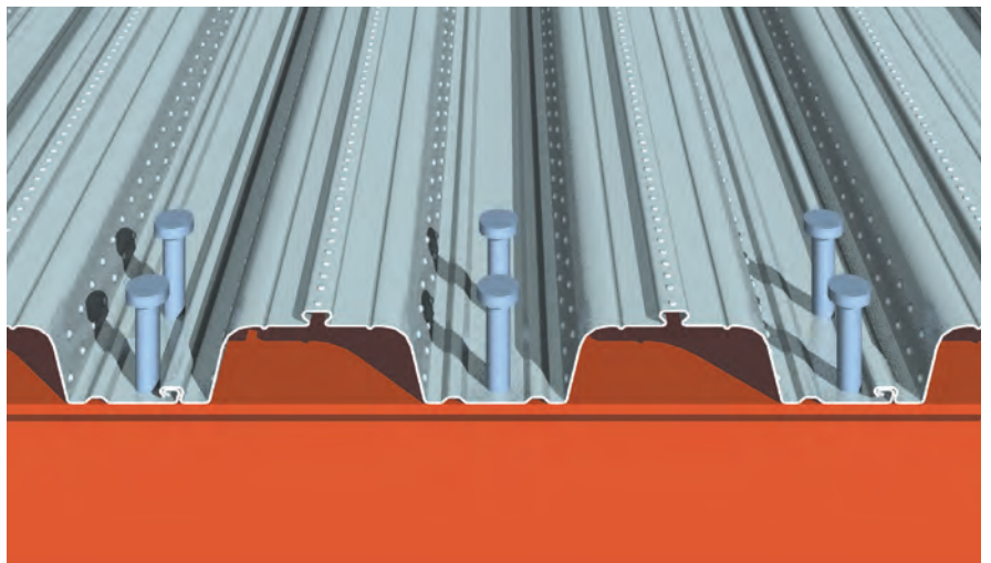
Centrally placed studs on CF 80
