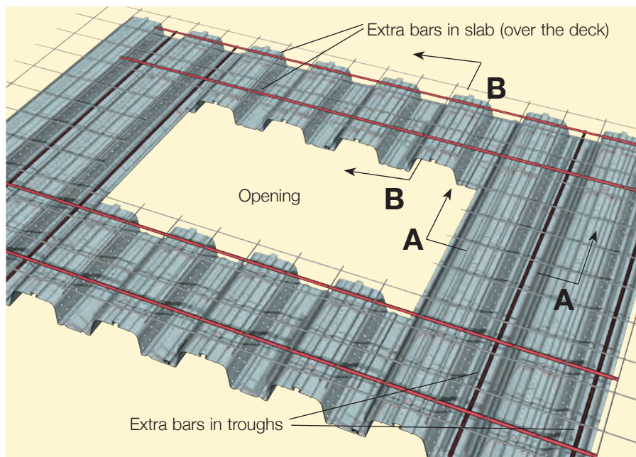
Reinforcement around opening
