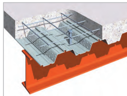
ComFlor 60
