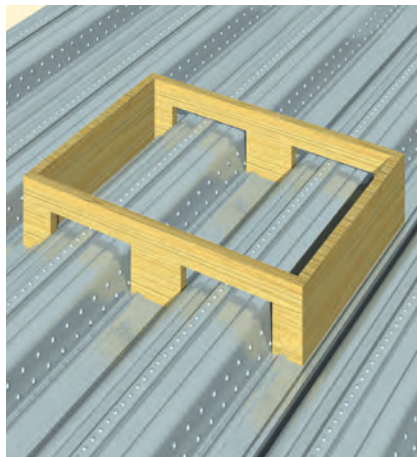
Timber shutter
