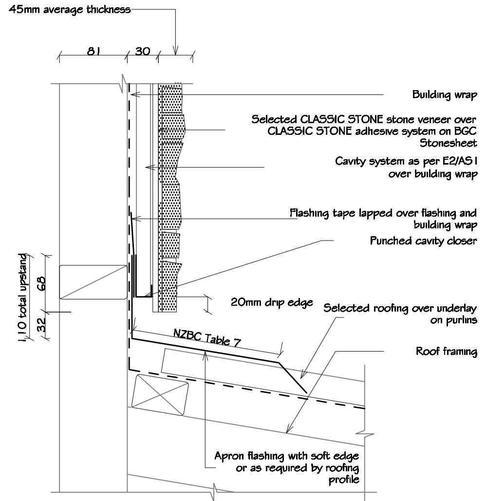
10 - Typical Roof Abutment Detail
