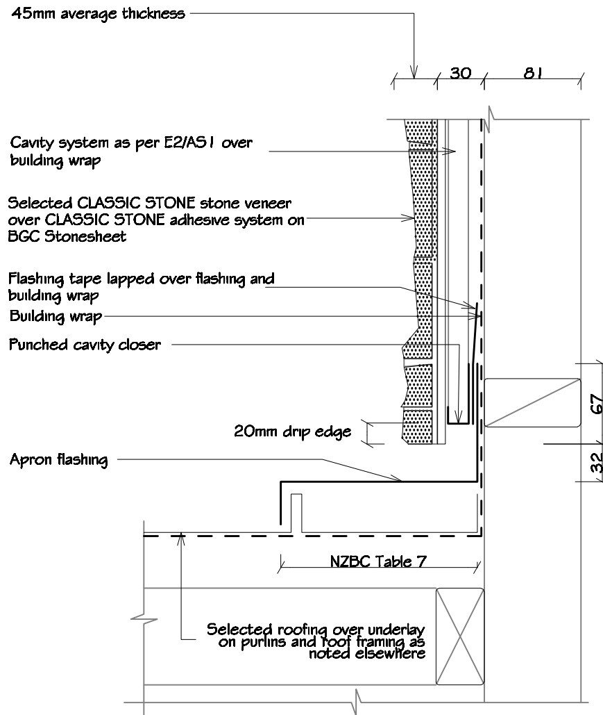
10 - Typical Roof Abutment Detail
