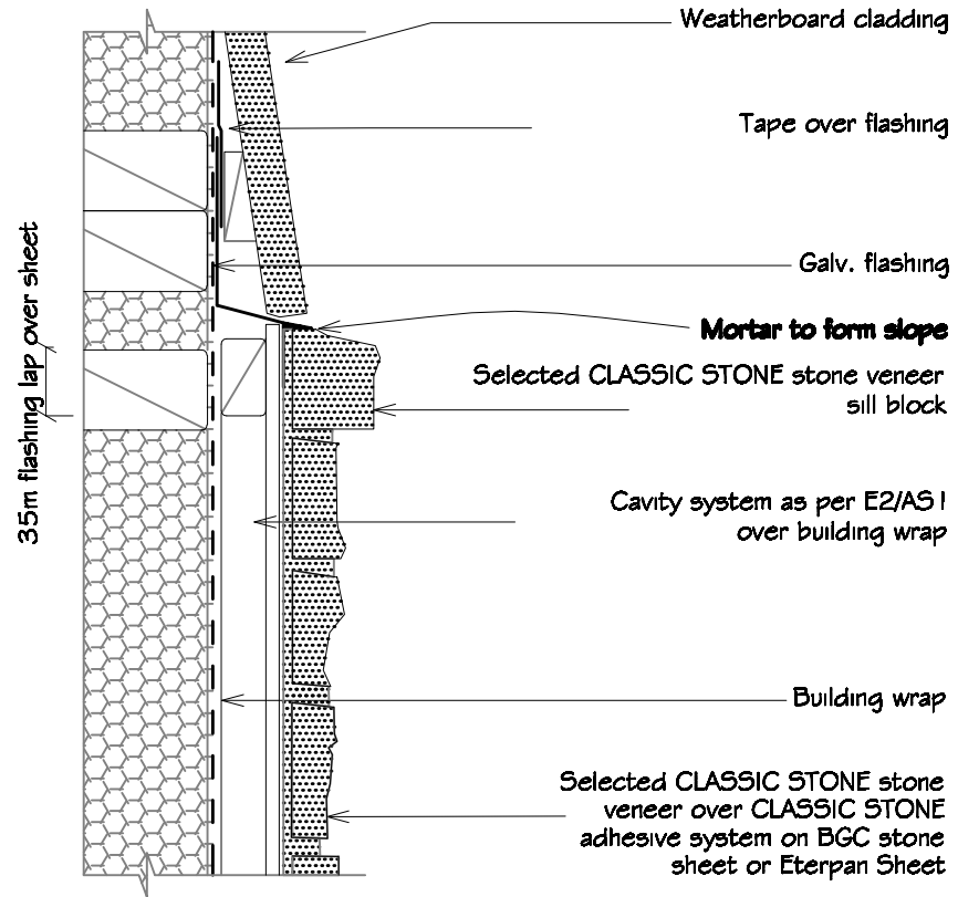
Alternative Sill Detail
