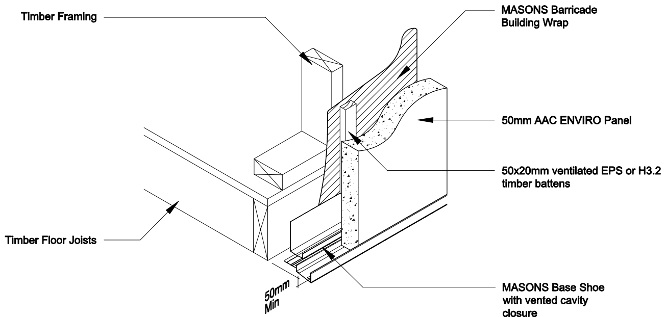
TIMBER FOOTING 3D View
