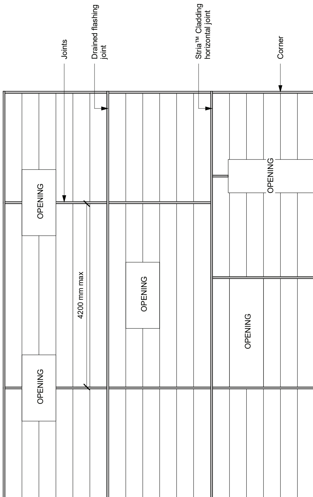
Figure 2: Vertical joint layout
