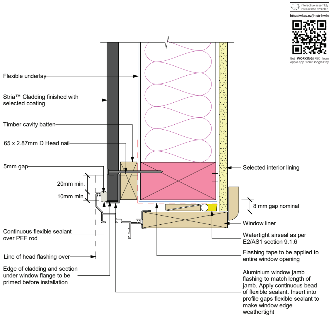
Figure 16: Window jamb
