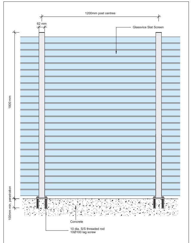
Glassvice Slat Screen Concrete Top Fix Elevation Date: 16/11/16 Scale: 1:10 Draft 02 Quick Code: QS110 © 2016. The copyright of this document is the property of Glass Vice Limited and shall not be reproduced, copied, loaned or disposed of directly or indirectly, nor used for any purpose other than that for which it is specifically licensed without prior consent. All dimensions in millimetres www.glassvice.com Phone +64 9 414 6565 info@glassvice.com
