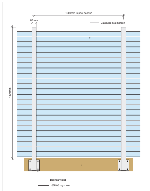
Glassvice Slat Screen Timber Side Fix Elevation Date: 16/11/16 Scale: 1:10 Draft 02 Quick Code: QS410 © 2016. The copyright of this document is the property of Glass Vice Limited and shall not be reproduced, copied, loaned or disposed of directly or indirectly, nor used for any purpose other than that for which it is specifically licensed without prior consent. All dimensions in millimetres www.glassvice.com Phone +64 9 414 6565 info@glassvice.com
