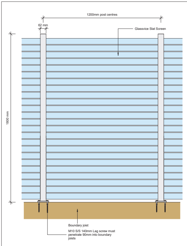
Glassvice Slat Screen Timber Top Fix Elevation Date: 16/11/16 Scale: 1:10 Draft 02 Quick Code: QS210 © 2016. The copyright of this document is the property of Glass Vice Limited and shall not be reproduced, copied, loaned or disposed of directly or indirectly, nor used for any purpose other than that for which it is specifically licensed without prior consent. All dimensions in millimetres www.glassvice.com Phone +64 9 414 6565 info@glassvice.com
