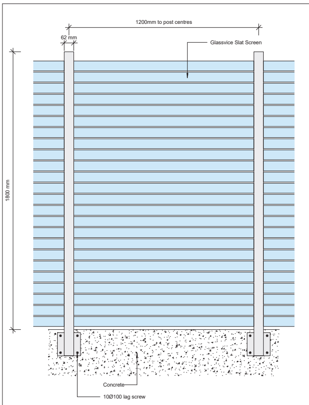
Glassvice Slat Screen Concrete Side Fix Elevation Date: 16/11/16 Scale: 1:10 Draft 02 Quick Code: QS310 © 2016. The copyright of this document is the property of Glass Vice Limited and shall not be reproduced, copied, loaned or disposed of directly or indirectly, nor used for any purpose other than that for which it is specifically licensed without prior consent. All dimensions in millimetres www.glassvice.com Phone +64 9 414 6565 info@glassvice.com
