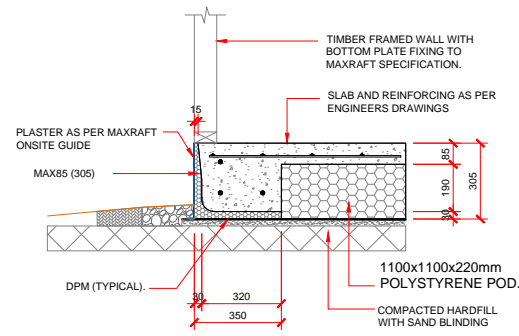
EXTERNAL FOOTING DETAIL 15mm TAPERED - 30mm BOTTOM
