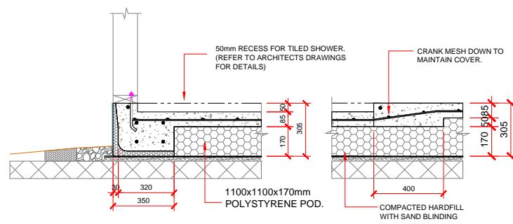
SHOWER RECESS DETAIL - 140mm FRAMING.
