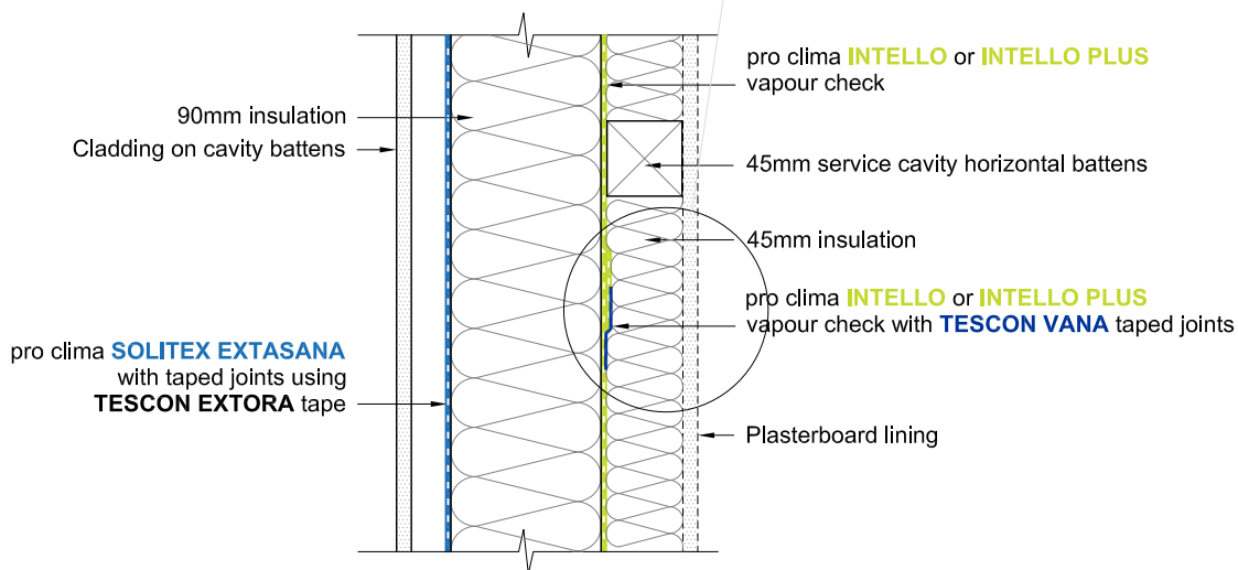
ELEVATION, 90mm WALL, WITH SERVICE CAVITY Scale 1:5 @ A4
